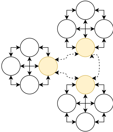
Figure 8 – Hierarchy: Steward
