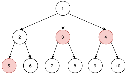
Figure 14 – Generic Tree
