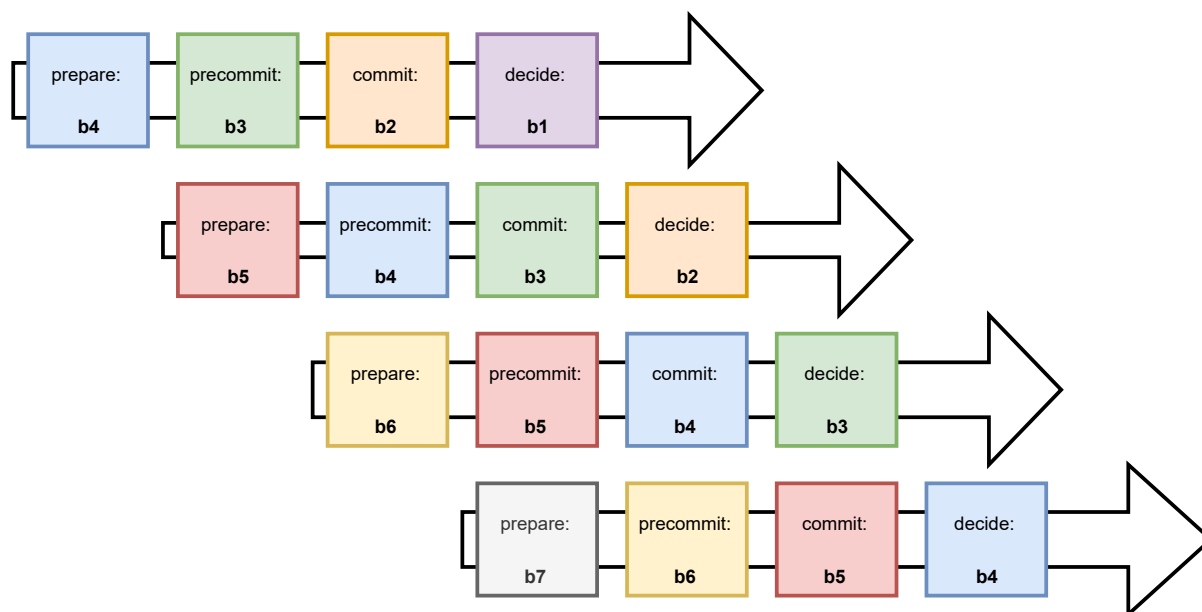
Figure 7 – HotStuff: Pipelining
