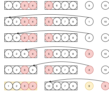
Figure 15 – Bin rotation
