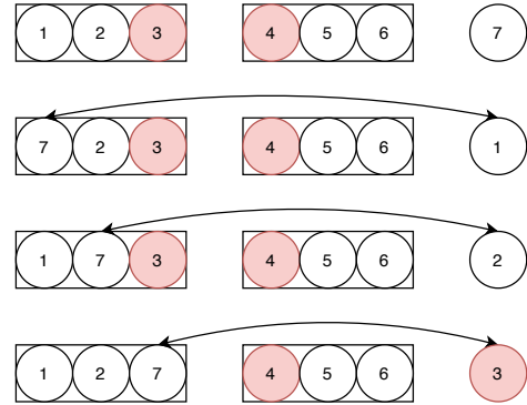
Figure 13 – Bin rotation
