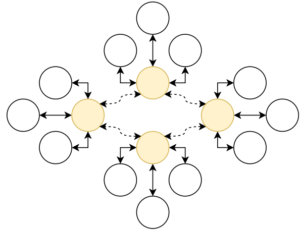
Figure 9 – Hierarchy: Fireplug
