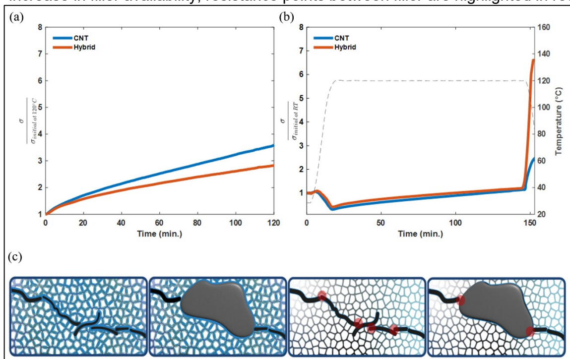
Figure 24 – (a) Evolution of EC ratio as function of time relative to the EC at the initial temperature of 120 °C (b) and the full test with the EC ratio evolution relative at room temperature. The grey dashed line shows the temperature change during the test, (c) a comparison of before and after annealing in the solid state shows the changes in crystallinity with the decrease of the amorphous phase (in blue) and the increase in filler availability, resistance points between filler are highlighted in red
