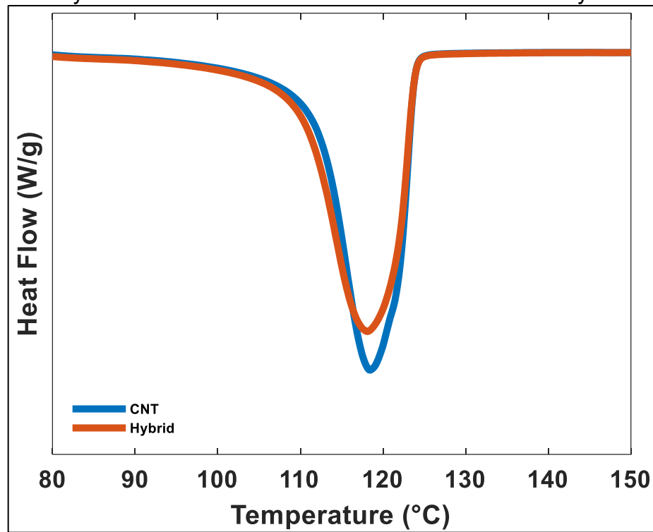
Figure 40 – Crystallization behaviour of HDPE/CNT and HDPE/Hybrid composites
