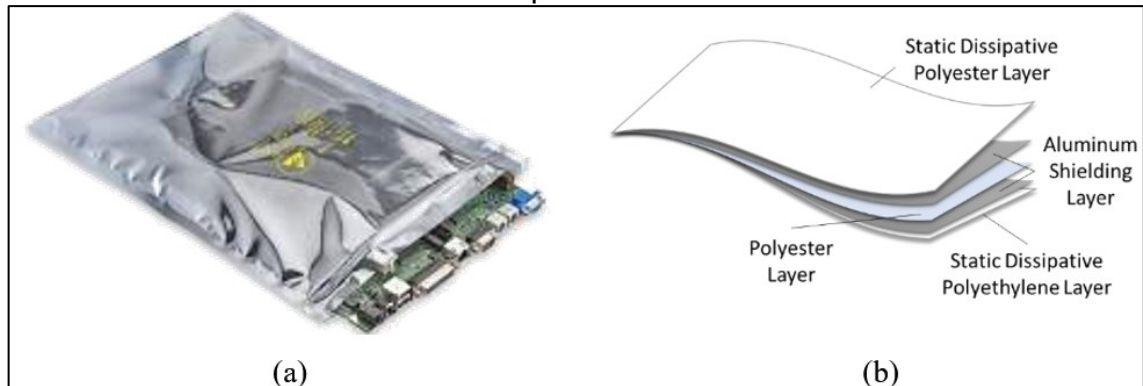
Figure 1 – (a) An electronic device protected by a flexible packaging ensuring protecting during transport, against moisture, electrostatic discharges and electromagnetic interference. (b) A multilayer structure of a commercial packaging solution to protect electronics
