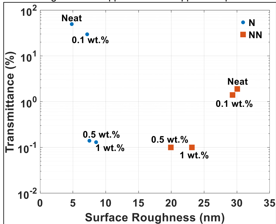
Figure 13 – Percentage of transmitted light in 500 nm as function of surface roughness for nipped and non-nipped samples
