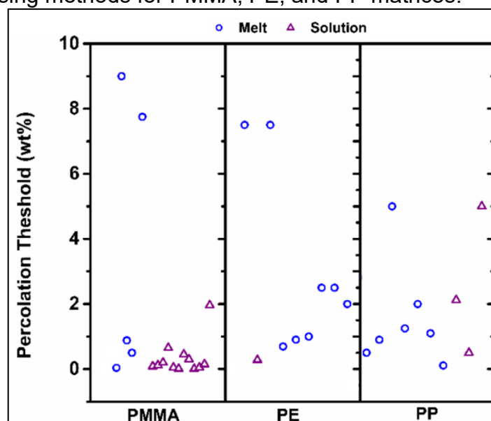
Figure 9 – Percolation threshold for different carbon nanotube/polymer composites for two processing methods for PMMA, PE, and PP matrices.
