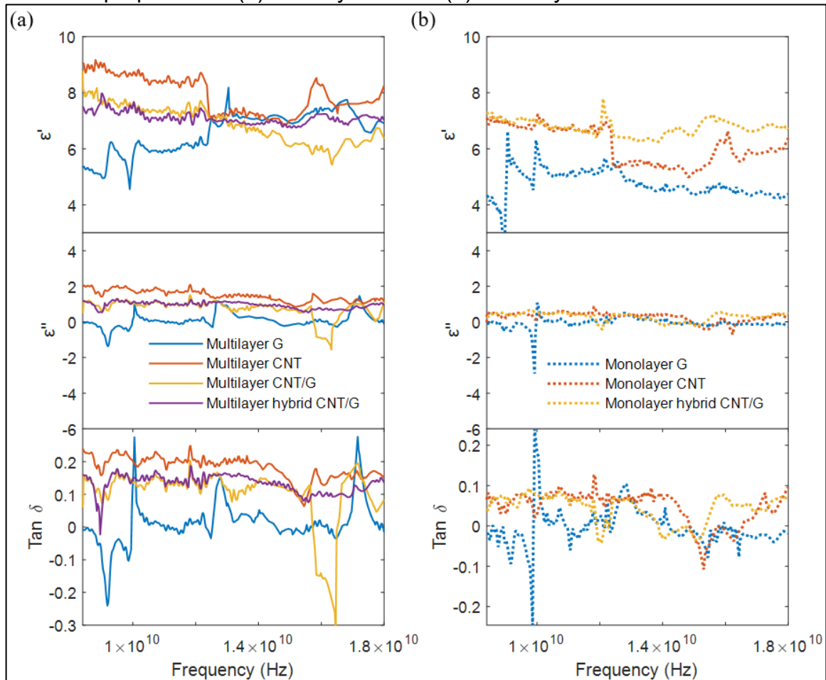
Figure 30 – Real part of permittivity, imaginary part of permittivity, and loss tangent properties of (a) multilayered and (b) monolayered flexible films
