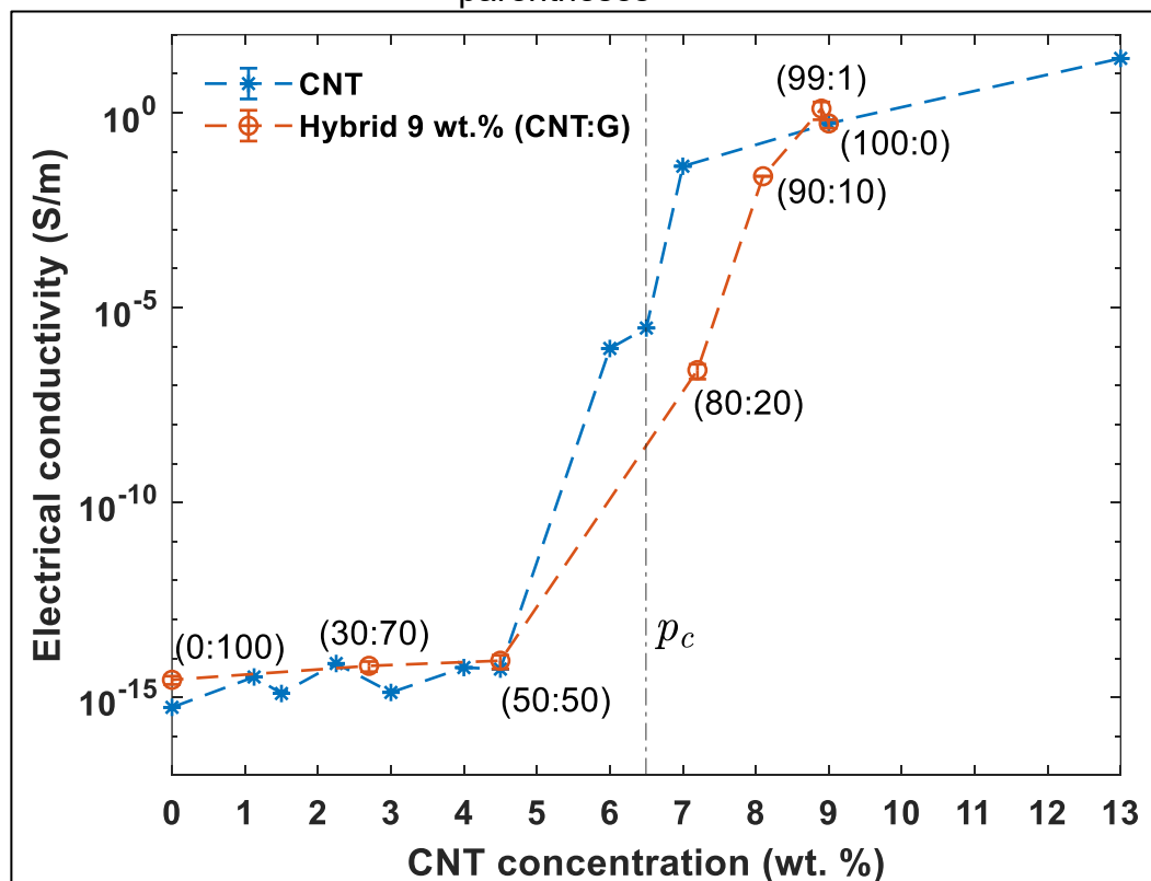
Figure 18 – Electrical conductivity as function of CNT concentration for CNT and hybrid composites. The respective weight percentage ratio of CNT:G are given in parentheses
