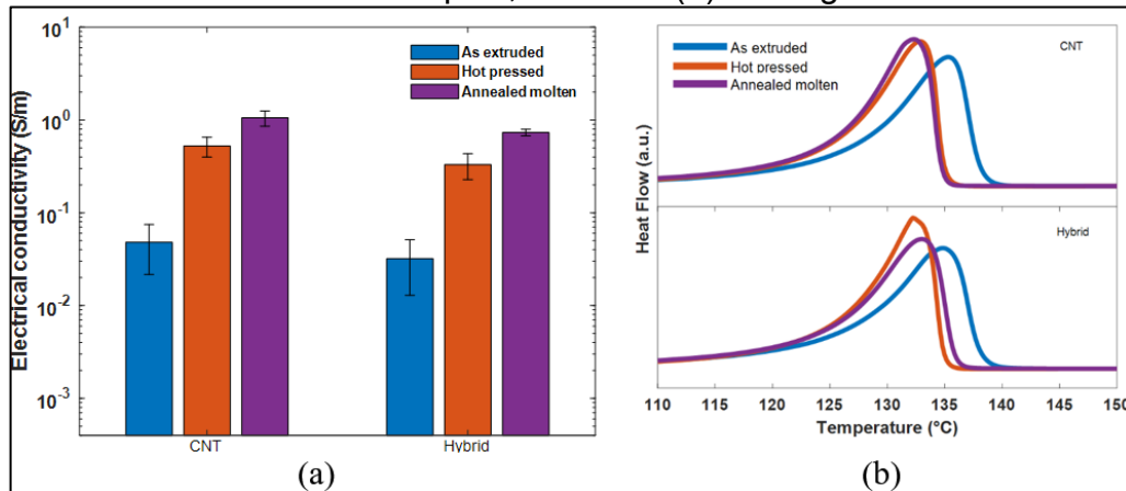
Figure 21 – (a) EC comparison between as obtained by extrusion, hot pressed and heat-treated samples, and their (b) melting behavior
