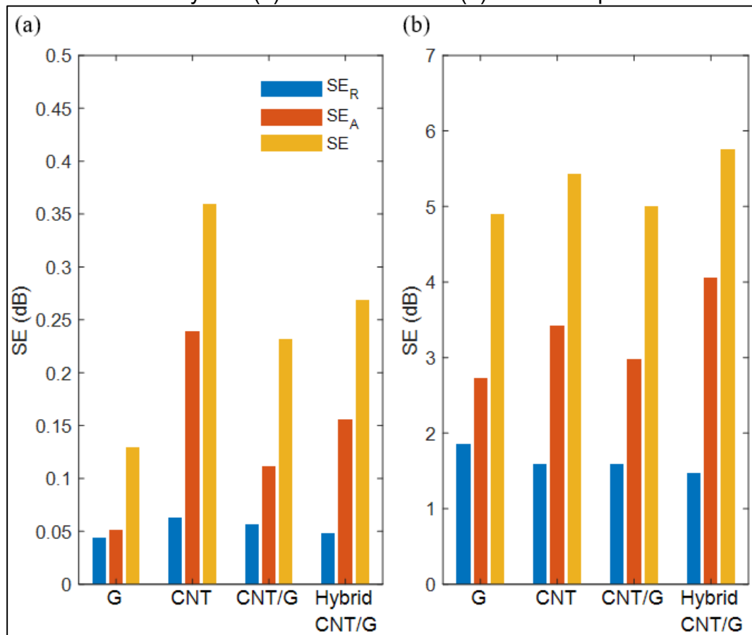
Figure 33 – Shielding by reflection and absorption and shielding effectiveness for multilayered (a) flexible films and (b) sheet samples
