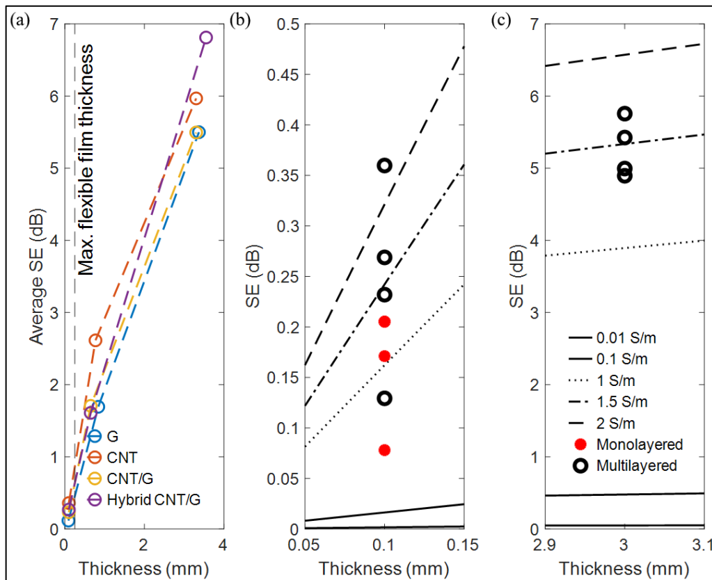
Figure 32 – (a) Experimental average SE as function of thickness, and compared to theoretical shielding effectiveness of (b) flexible films (c) sheet samples for specific electrical conductivities
