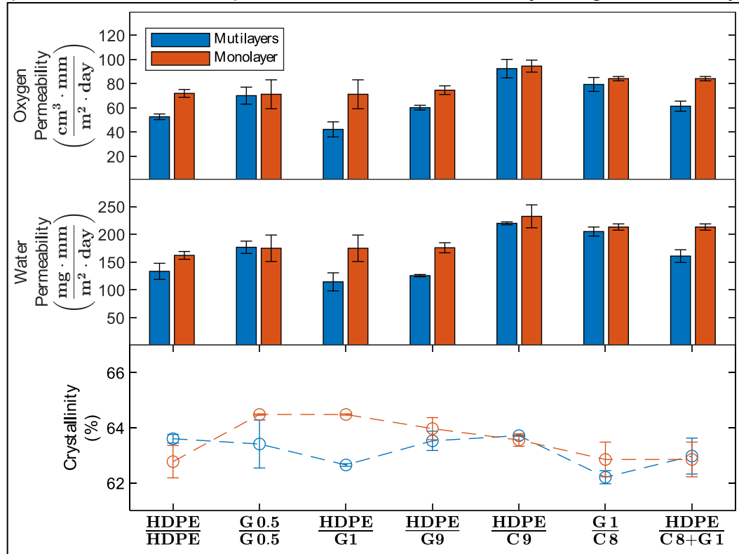
Figure 28 – Water and oxygen permeability and respective crystallinities for the investigated structures. Each structure type is shown in the bottom of the figure, where Layer A is represented on top and Layer B on the bottom. The same compositions were used for the monolayered films. The average crystallinities are provided for each composition, the dashed lines are just a guide to the eye
