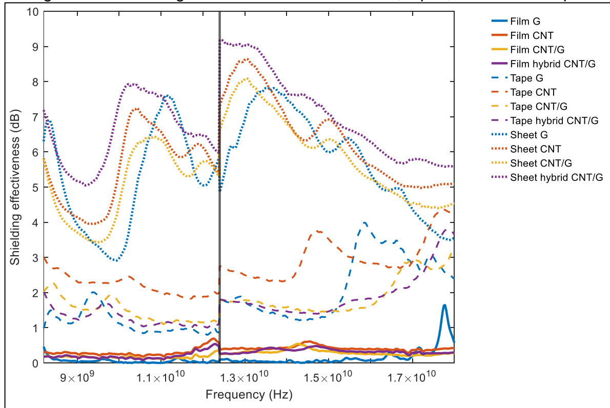
Figure 31 – Shielding effectiveness of flexible films, tapes, and sheet samples
