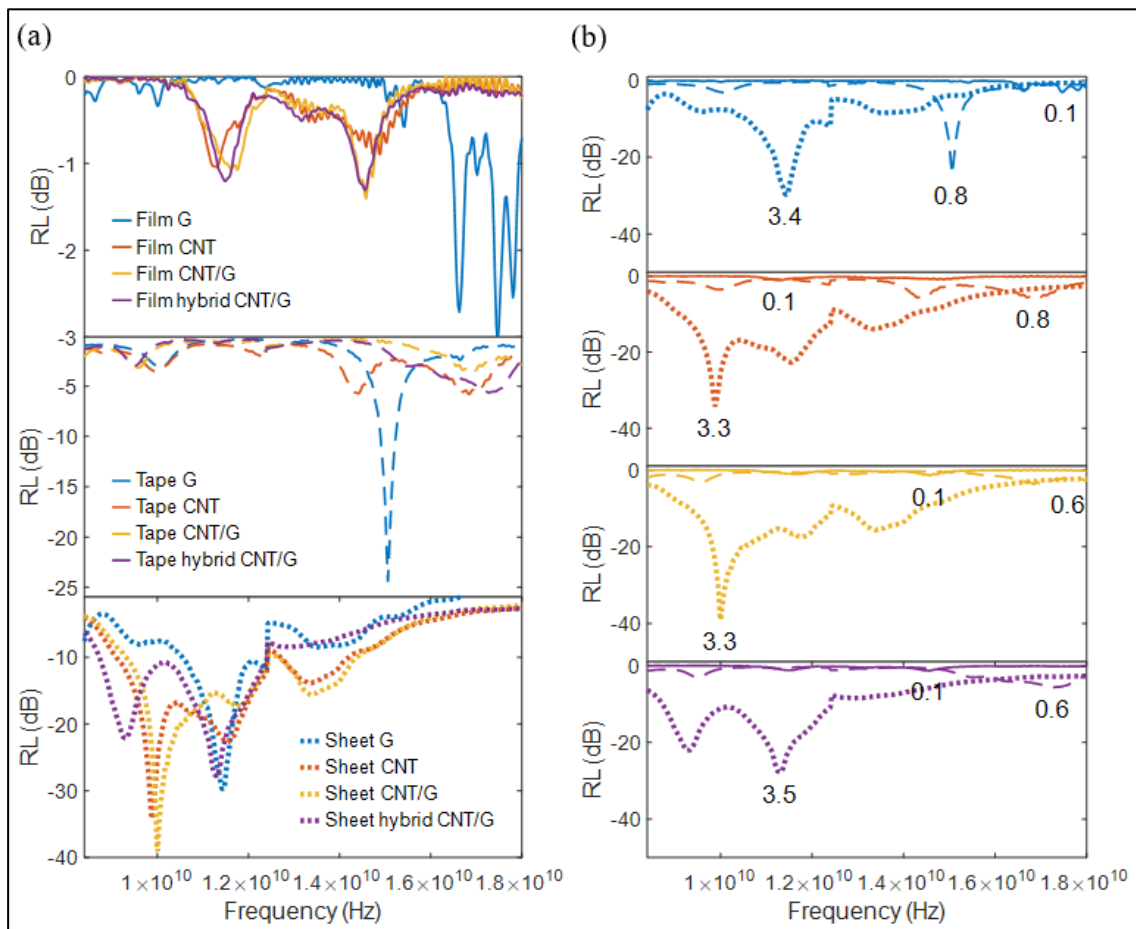
Figure 34 – RL for grouped by similar (a) thickness, namely, films, tape or sheet and (b) group type based on composition with the minimum peak of RL highlighted with the material thickness in mm
