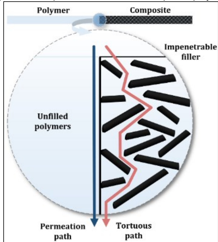
Figure 5 – Tortuosity effect with the addition of layered particles in a polymeric matrix on the right side compared to an unfilled amorphous polymer on the left side
