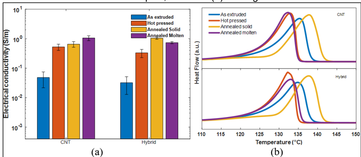
Figure 23 – (a) EC comparison between as obtained by extrusion, hot pressed and heat-treated samples, and their (b) melting behavior
