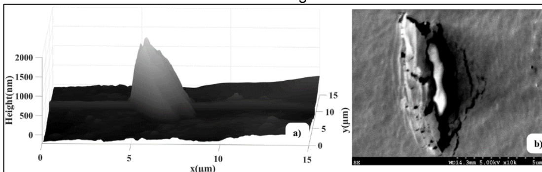
Figure 38 – a) AFM mapping in height mode and b) SEM picture where both shows filler defects at the surface of the 1 wt.% composite films induced by surface finishing
