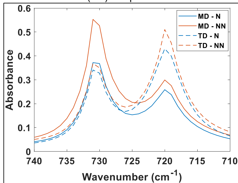
Figure 39 – Polarized FTIR spectra in MD and TD for nipped (N) and non-nipped (NN) composites
