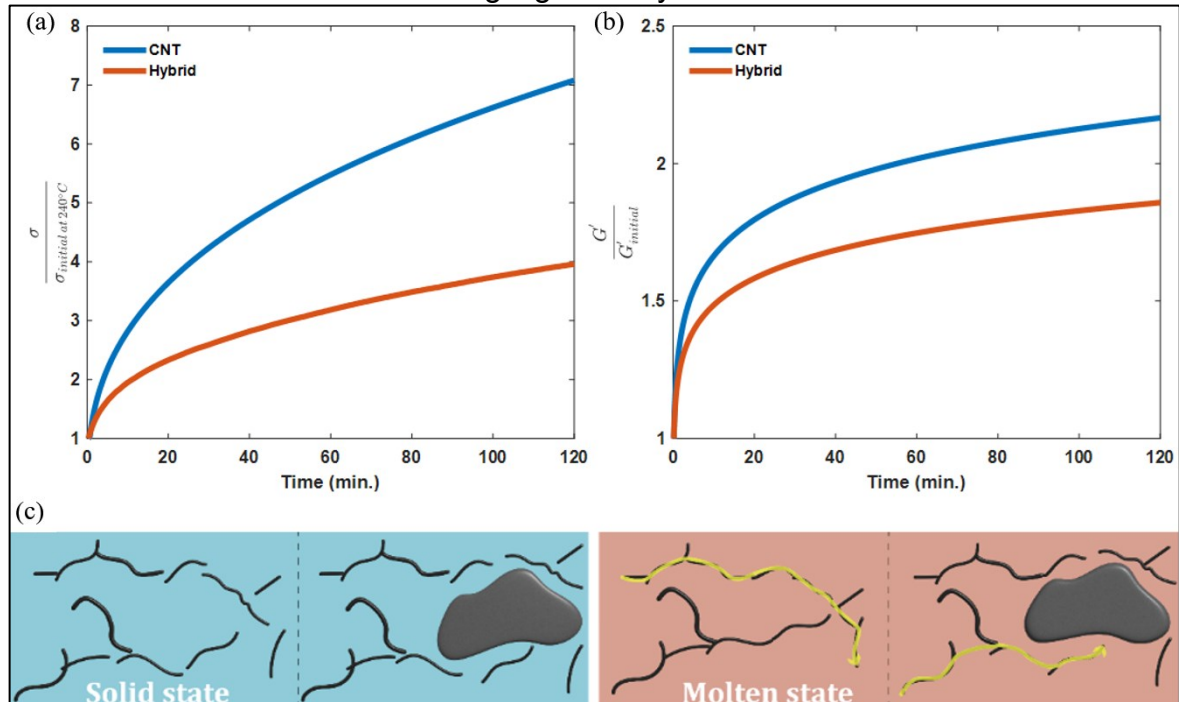
Figure 22 – (a) EC evolution ratio relative to treatment temperature (240 °C) and (b) complex storage modulus ratio as a function of time for each group of sample, (c) a comparison of the effect of the G (larger particle) addition on the CNT (tubes) network reorganization with annealing in the molten state, an electrical path, is highlighted in yellow
