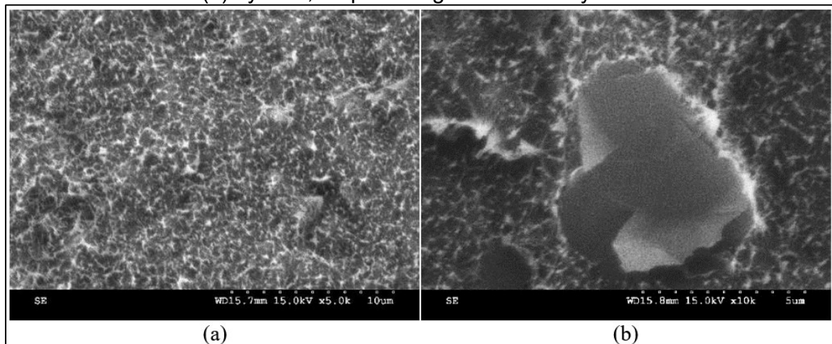
Figure 20 – SEM imaging of composites morphology containing (a) only CNT and (b) hybrids, emphasizing the secondary filler
