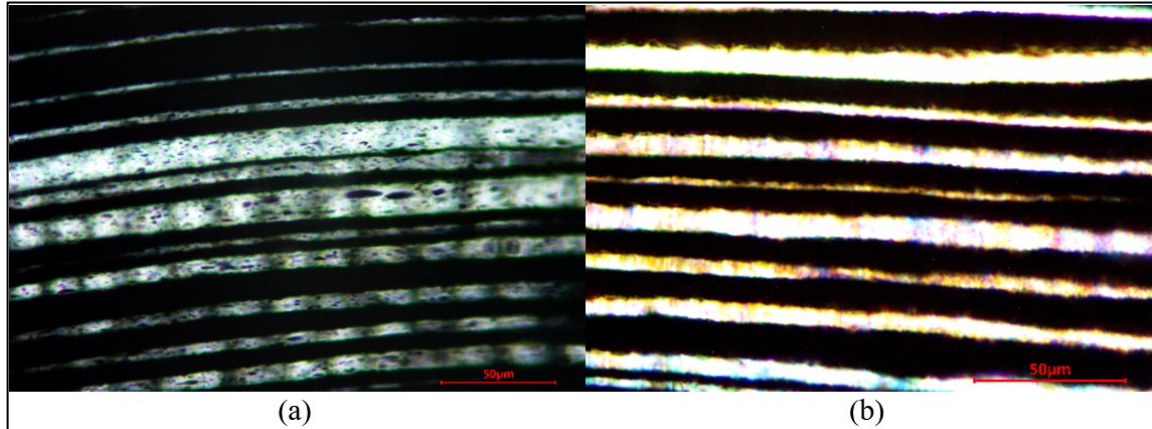
Figure 27 – Multilayered tapes with (a) alternating layers of HDPE/0.5 wt.% G and HDPE/4 wt.% CNT, and (b) alternating layers of HDPE/CNT/G with a 4.5% wt.% loading
