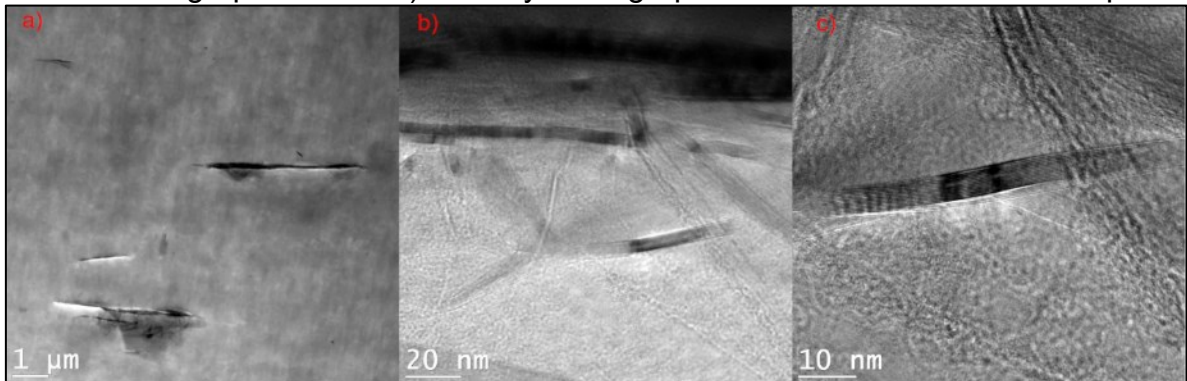
Figure 15 – TEM in the M-T plane showing a) primary agglomerates, b) non-exfoliated graphene and c) Few layers of graphene in the 0.5 wt.% NN composite
