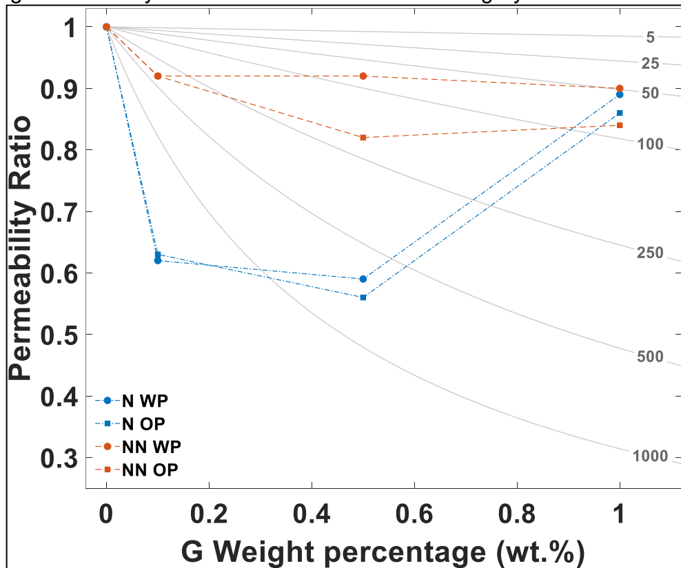
Figure 16 – Permeability ratio as function of filler weight concentration for experimental and predicted data. The lines between the experimental data points are just a guide to the eyes. The indicated numbers in the grey lines are the used AR
