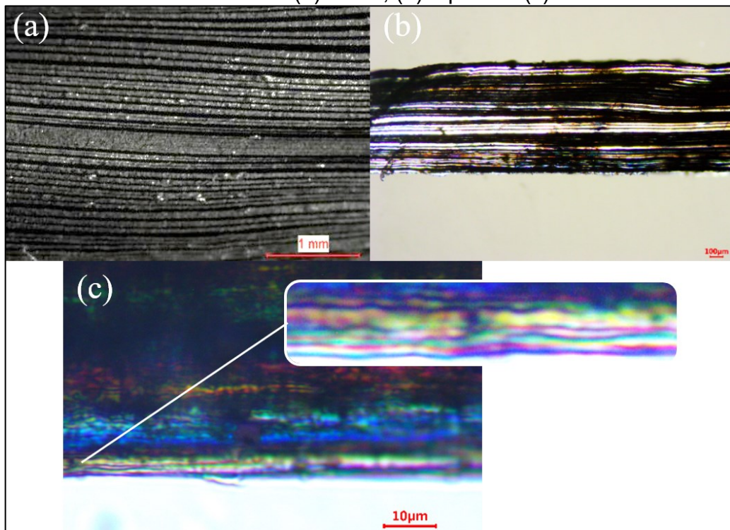
Figure 25 – Multilayered composites of HDPE/G with 4.5 wt.% filler content with different thicknesses (a) sheet, (b) tape and (c) flexible film
