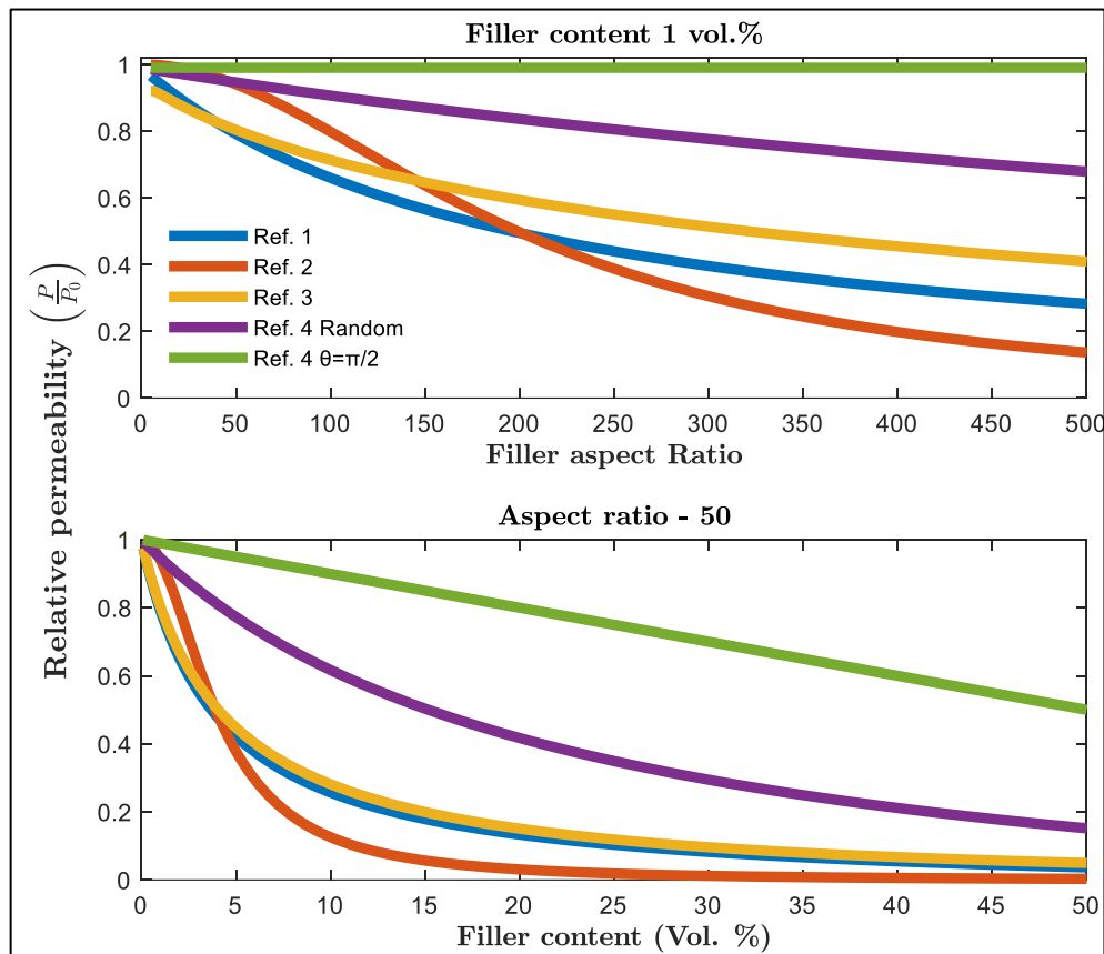
Figure 7 – Relative permeability predictions for a filler content of 1 vol.% as a function of filler AR and for a fixed AR = 50 as a function of filler volume content
