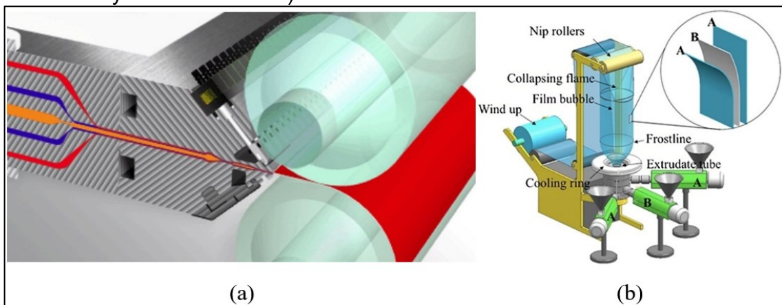
Figure 11 – Coextrusion techniques a) cast film extrusion with a cross section showing the joining of different flows highlighted in different colors forming a final multilayered film and a b) blown film extrusion line with an ABA structure
