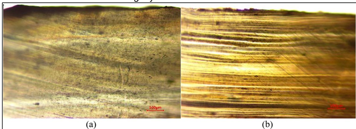
Figure 26 – Multilayered tapes (a) with only layers composed of 0.5 wt.% G (b) alternating layers of HDPE and 1 wt.% G
