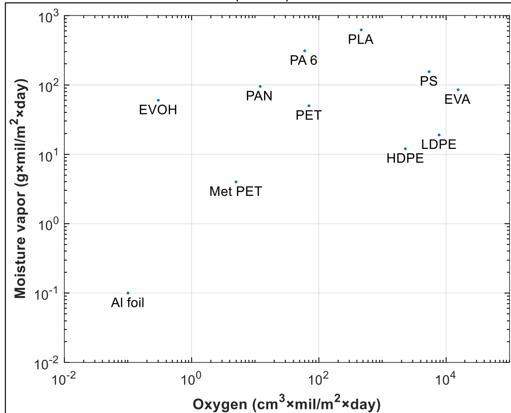
Figure 2 – Values of moisture vapor transmission rate at 38°C, 90% Relative humidity (RH) and oxygen permeation at 23°C, 0% RH of different packaging materials. Where abbreviations stand for, Aluminum (Al); ethylene vinyl acetate (EVA); high-density polyethylene (HDPE); low-density polyethylene (LDPE); Polyacrylonitrile (PAN); Metalized (Met); polyamide (PA); polyethylene terephthalate (PET); polylactide (PLA); polystyrene (PS); ethylene-vinyl alcohol copolymer (EVOH).
