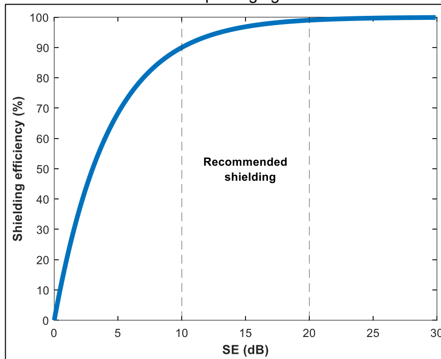
Figure 10 – Shielding efficiency as function of SE including the recommended values for a packaging material
