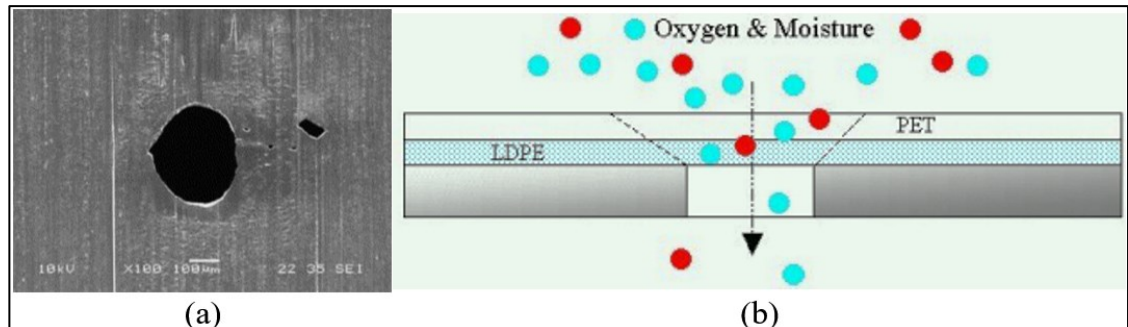
Figure 3 – (a) Pinholes caused in an aluminum foil during its lamination process observed under a scanning electrical microscope (SEM) and (b) Representation of oxygen and moisture diffusion through a pinhole in a PET/ LDPE/ Foil packaging material.
