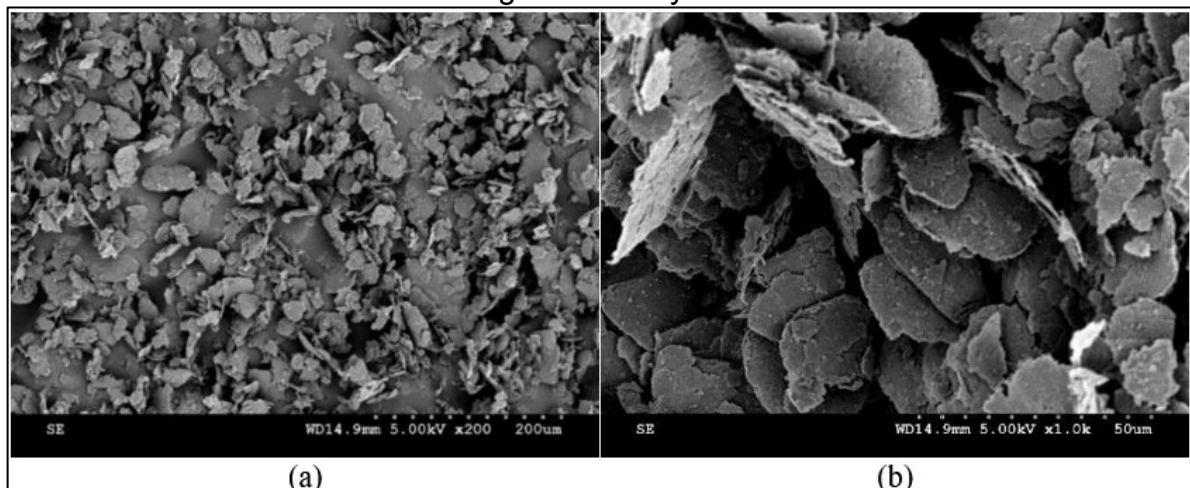
Figure 19 – Powder morphology of graphene at (a) 200x and (b) 1000x times magnification by SEM
