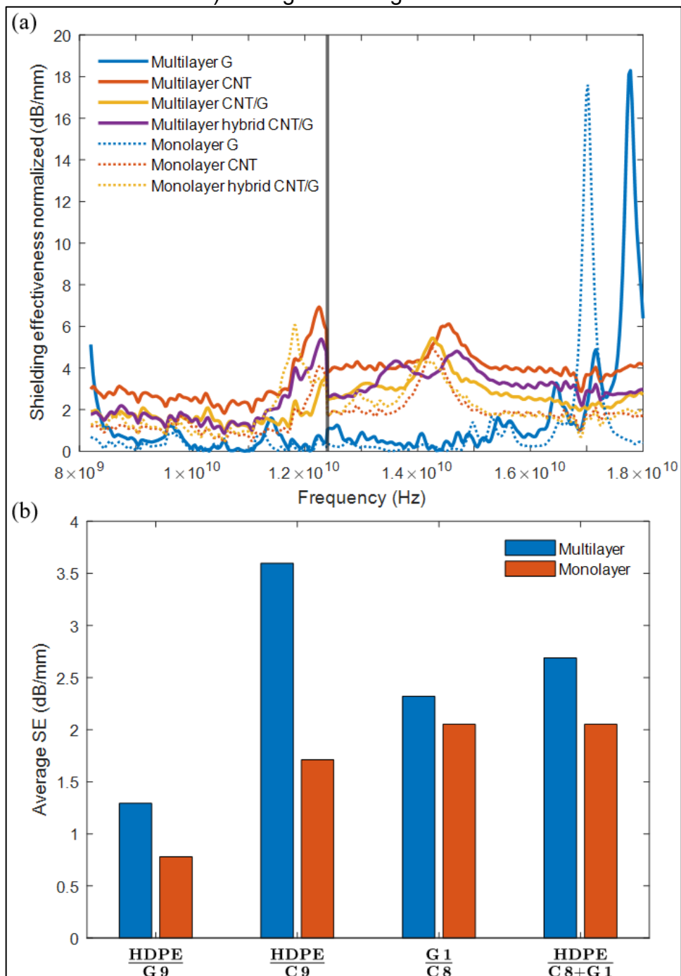
Figure 29 – Multilayered and monolayered flexible films a) shielding effectiveness normalized and b) average shielding effectiveness normalized
