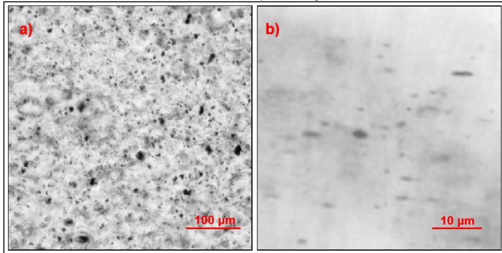
Figure 36 – Original OM pictures of NN 0.1 wt.% G a) top view and b) cross section view, respectively
