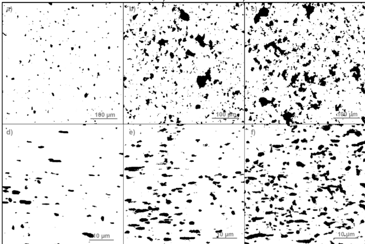
Figure 14 – The top row presents top view pictures of NN samples a) 0.1 wt.% G, b) 0.5 wt.% G and c) 1 wt.% G. The bottom row presents cross section pictures of d) 0.1 wt.% G, e) 0.5 wt.% G and f) 1 wt.% G
