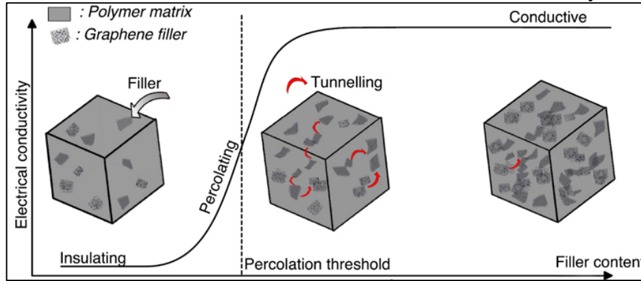
Figure 8 – Effect of the conductive filler content in an insulating polymer matrix. For small concentrations, the composite is insulating; above a critical amount of filler, there is a marked increase in the electrical conductivity
