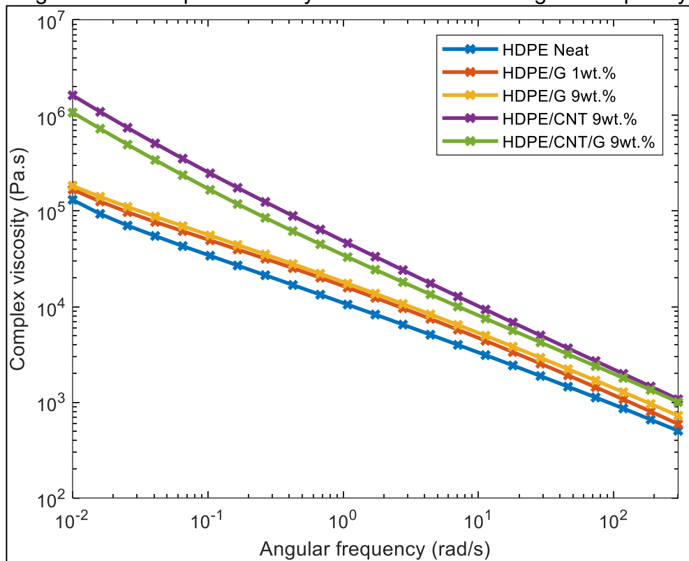
Figure 41 – Complex viscosity data as function of angular frequency
