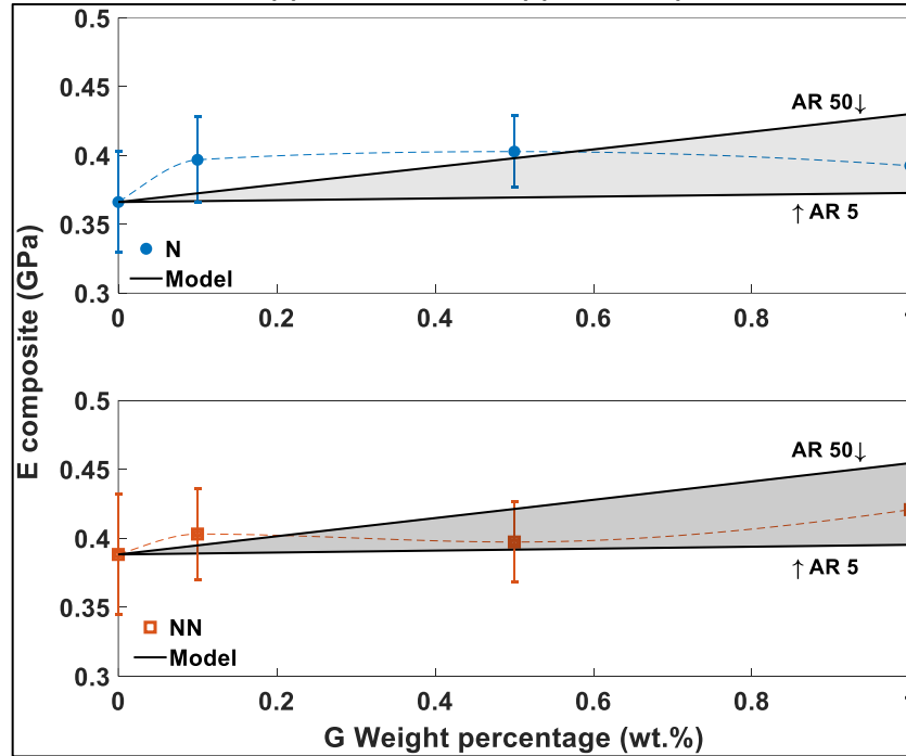
Figure 17 – Young’s modulus of composites and model with AR between 5 and 50 for nipped and non-nipped samples
