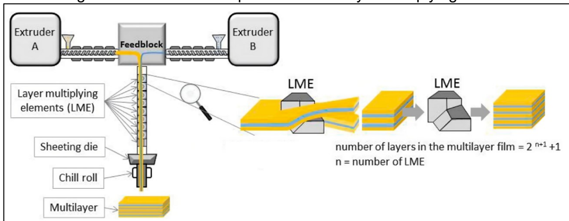
Figure 12 – Coextrusion process with a layer multiplying element
