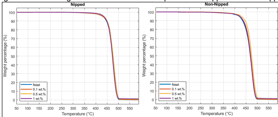
Figure 35 – Thermogravimetric of neat and composite films nipped and non-nipped
