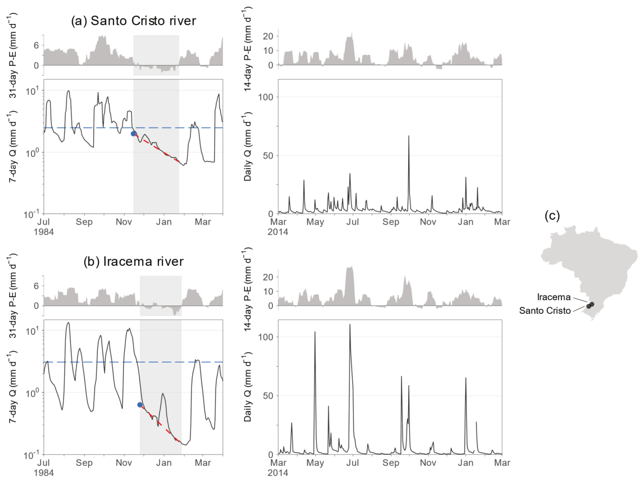
Figure 4.3. Low flow generation on a pair of basins with similar climate and geology but contrasting soils. Time series of streamflow (Q) and rainfall (P) minus evaporation (E) in the: (a) Santo Cristo river (high soil infiltration capacity), 346 \text{ km}^2 , gauge code 74750000; (b) Iracema river (low soil infiltration capacity), 300 \text{ km}^2 , gauge 74295000. Note the different Q and P – E scales between the left and right-hand-side panels. (c) Location map. The blue dashed lines show the mean annual streamflow. The shaded rectangles indicate dry spells. The red dashed lines show the streamflow fit during the dry spell and the blue circle shows the estimated initial flow.
